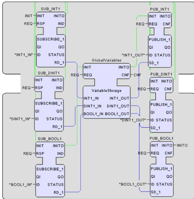
Fig. 17 Global/local Variable Composite Function Block.
