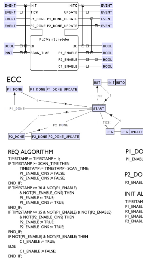
Fig. 5 Main Scheduler Interface, Execution Control Chart (ECC) and scheduling algorithms (for preemptive PLC execution semantics).
