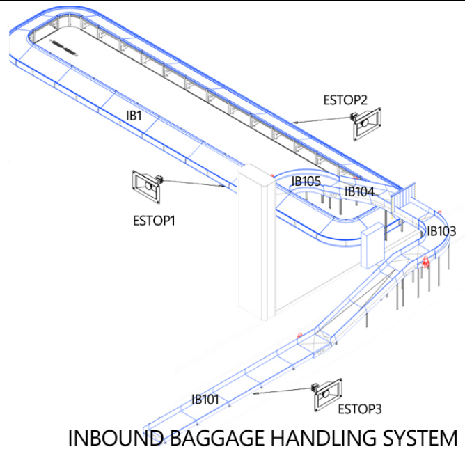
Fig. 18 Case study inbound baggage handling system layout.
