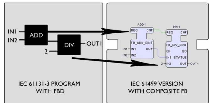
Fig. 16 IEC 61131-3 FBD mapping to IEC 61499 Composite FB.
