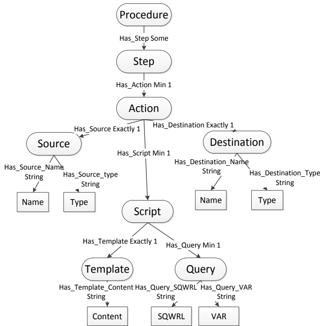
Fig. 7 Knowledge Base Definition for Migration Mapping Rules
